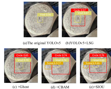
FIGURE 16. The visual results of the ablation study.
