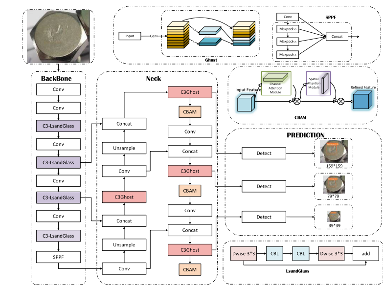
FIGURE 8. The improved YOLO Model (LCG-YOLO).
