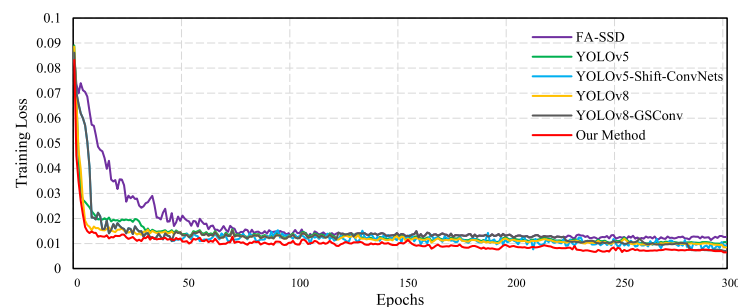
FIGURE 10. The training loss of different models.
