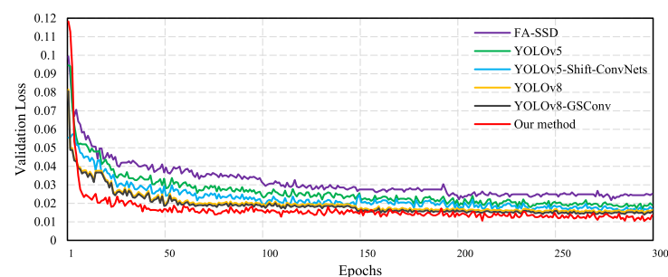
FIGURE 11. The validation loss of different models.
