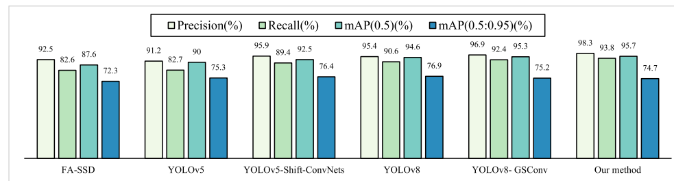
FIGURE 13. The Precision, Recall and mAP of different models.
