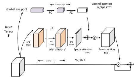
FIGURE 5. The CBAM structure diagram.
