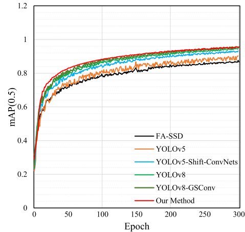
FIGURE 12. The mAP (0.5) iteration diagram for different models.
