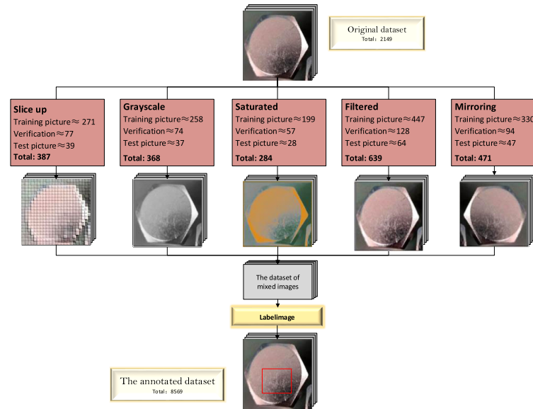
FIGURE 9. Data set and preprocessing.
