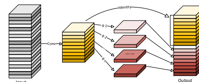
FIGURE 4. The ghost module.
