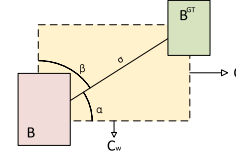
FIGURE 6. The scheme for calculation the contribution of the angle cost to the loss function.
